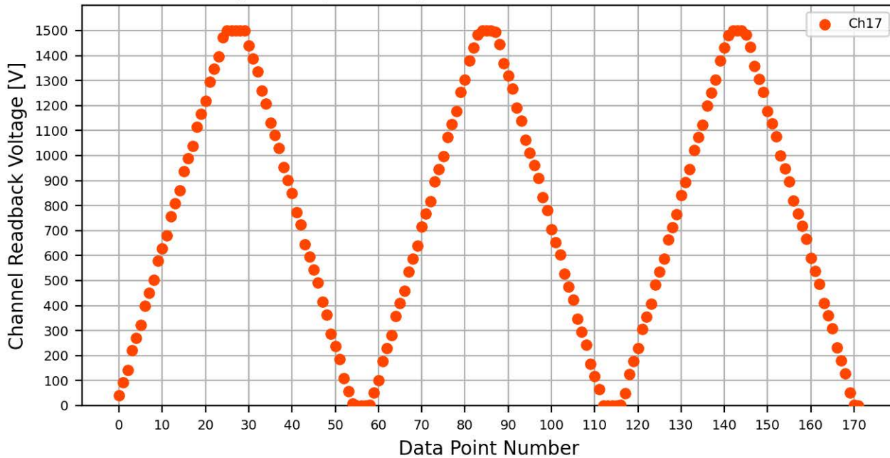
Voltage Ramp Test (Python) Bd #083, Slot #6, Ch #17
