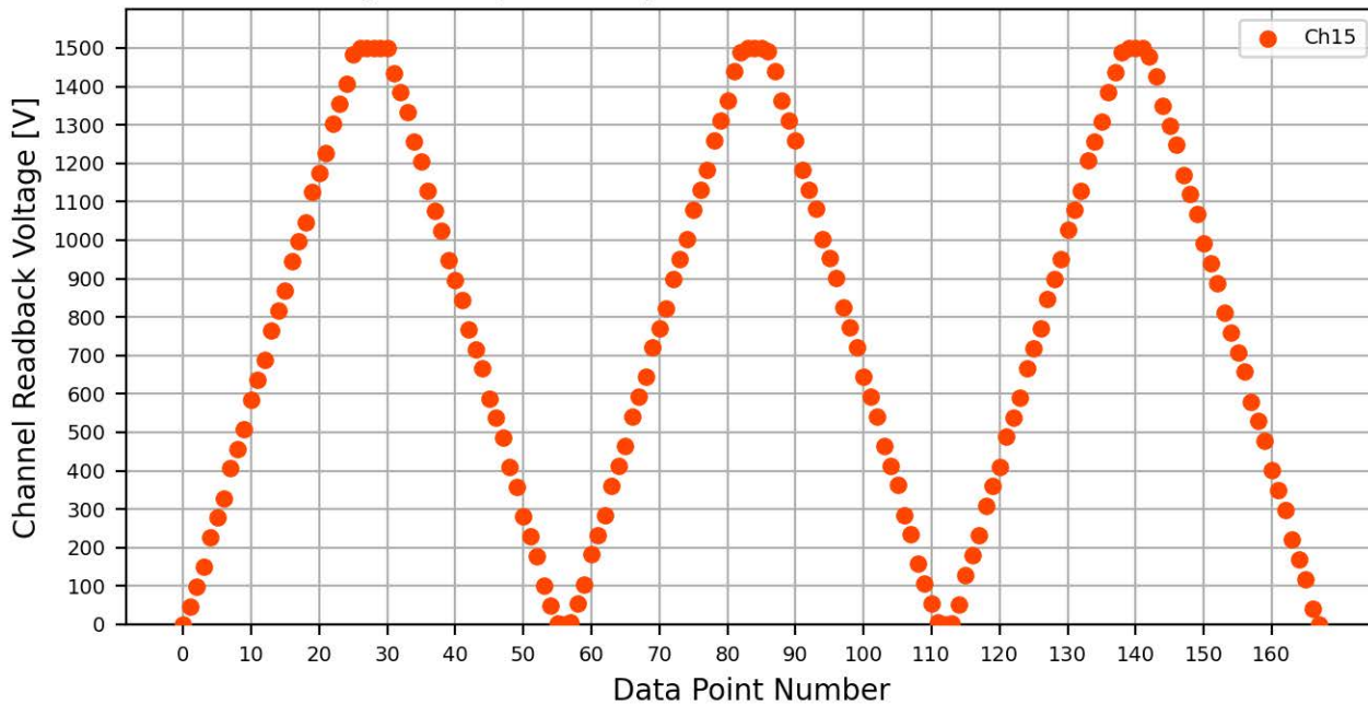
Voltage Ramp Test (Python) Bd #083, Slot #6, Ch #15
