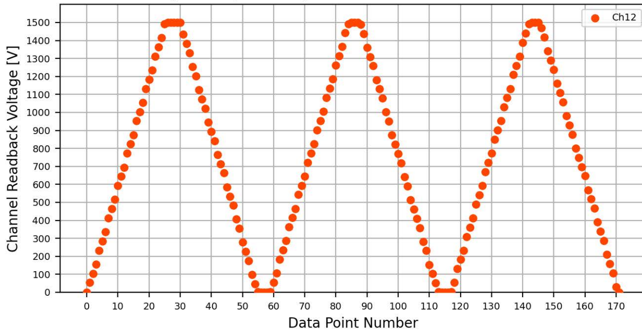
Voltage Ramp Test (Python) Bd #083, Slot #6, Ch #12
