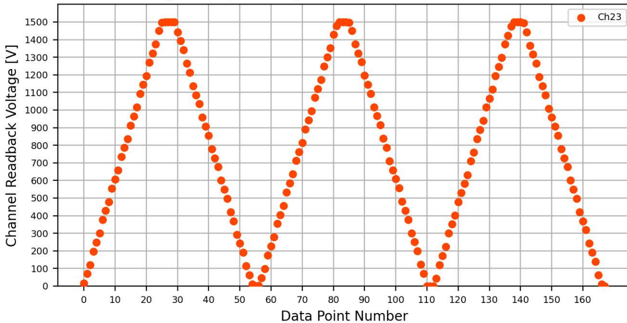
Voltage Ramp Test (Python) Bd #083, Slot #6, Ch #23
