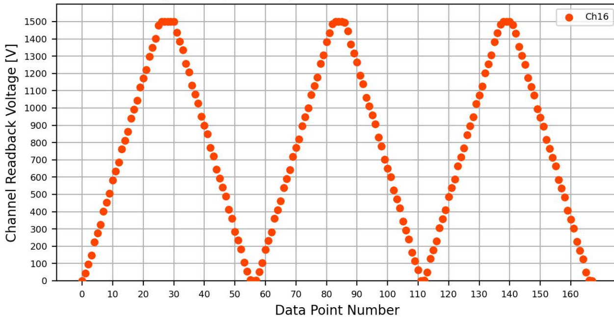
Voltage Ramp Test (Python) Bd #083, Slot #6, Ch #16
