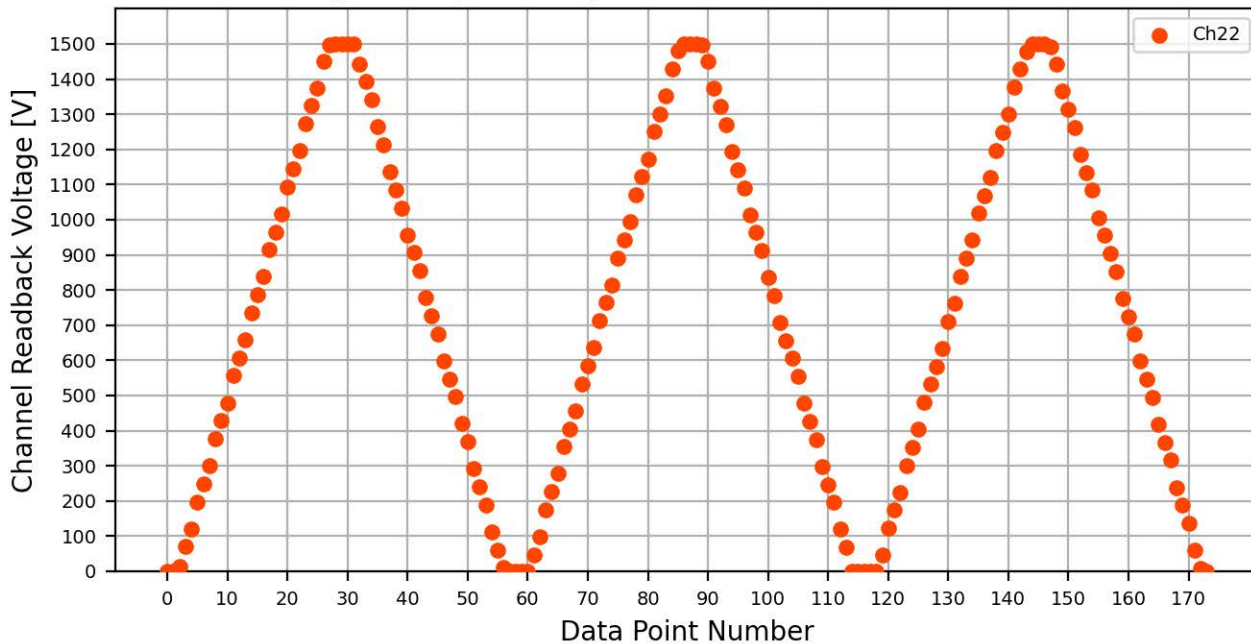
Voltage Ramp Test (Python) Bd #083, Slot #6, Ch #22
