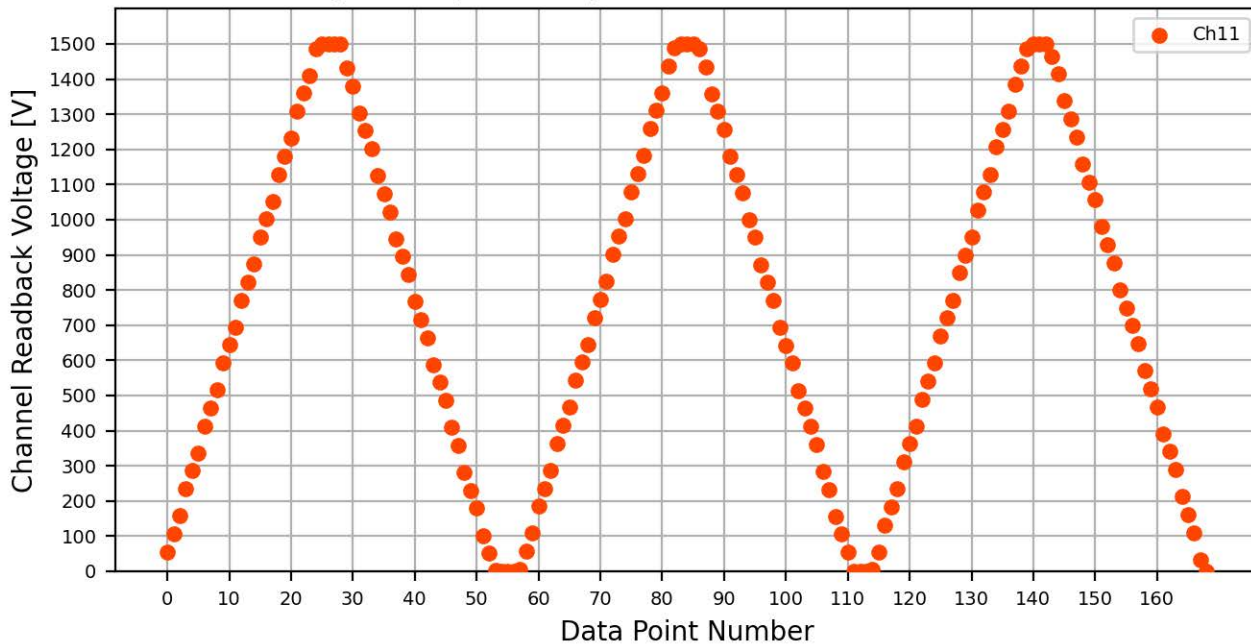
Voltage Ramp Test (Python) Bd #083, Slot #6, Ch #11
