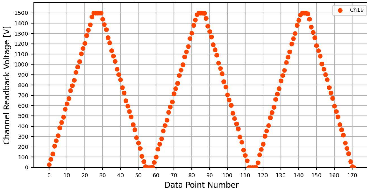
Voltage Ramp Test (Python) Bd #083, Slot #6, Ch #19
