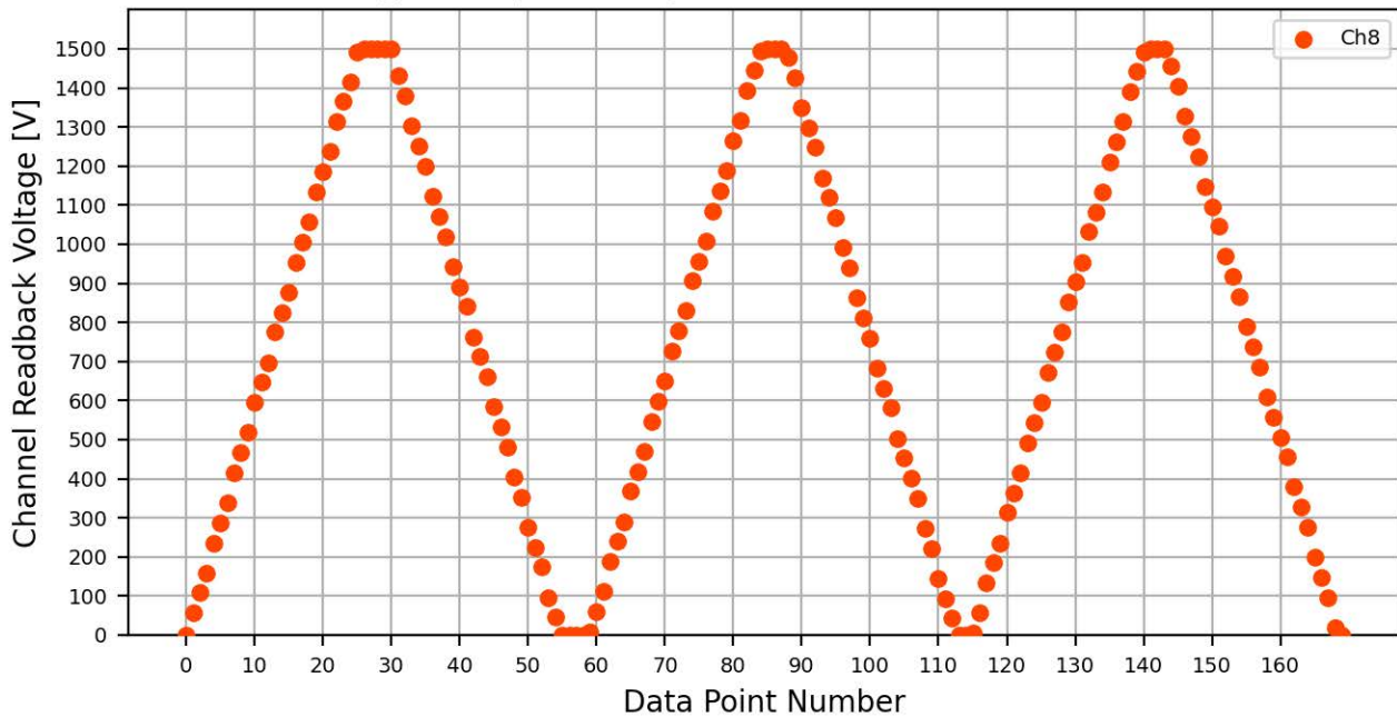
Voltage Ramp Test (Python) Bd #083, Slot #6, Ch #8
