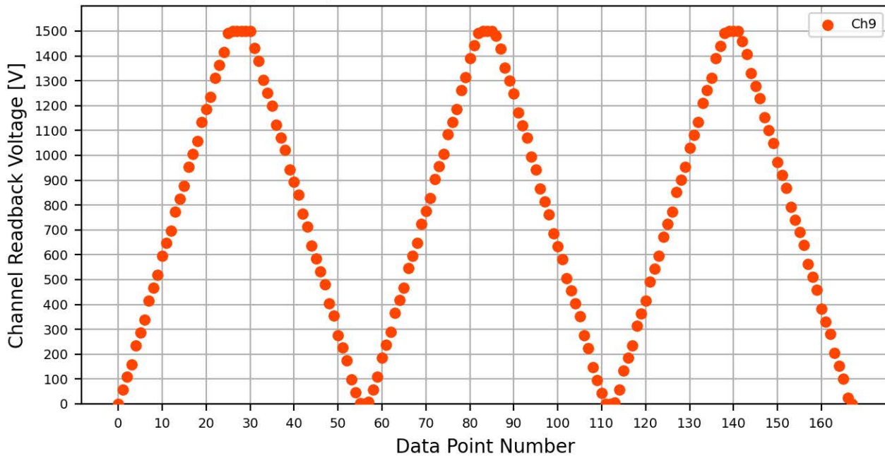
Voltage Ramp Test (Python) Bd #083, Slot #6, Ch #9
