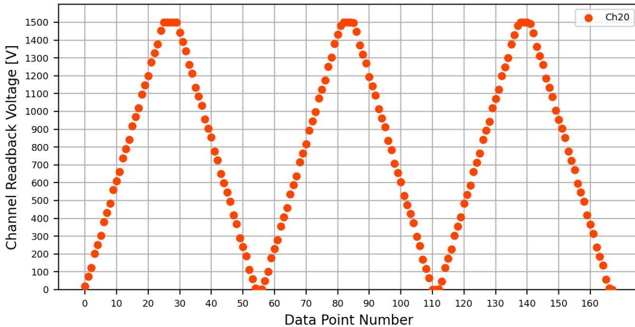
Voltage Ramp Test (Python) Bd #083, Slot #6, Ch #20
