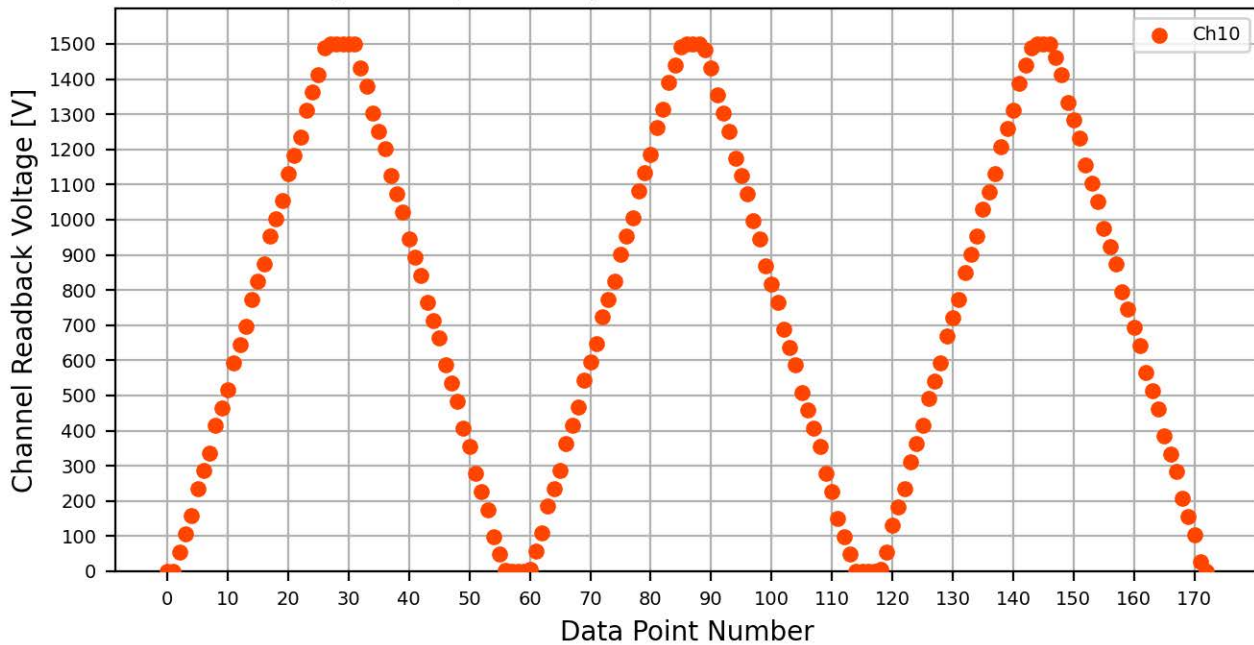
Voltage Ramp Test (Python) Bd #083, Slot #6, Ch #10
