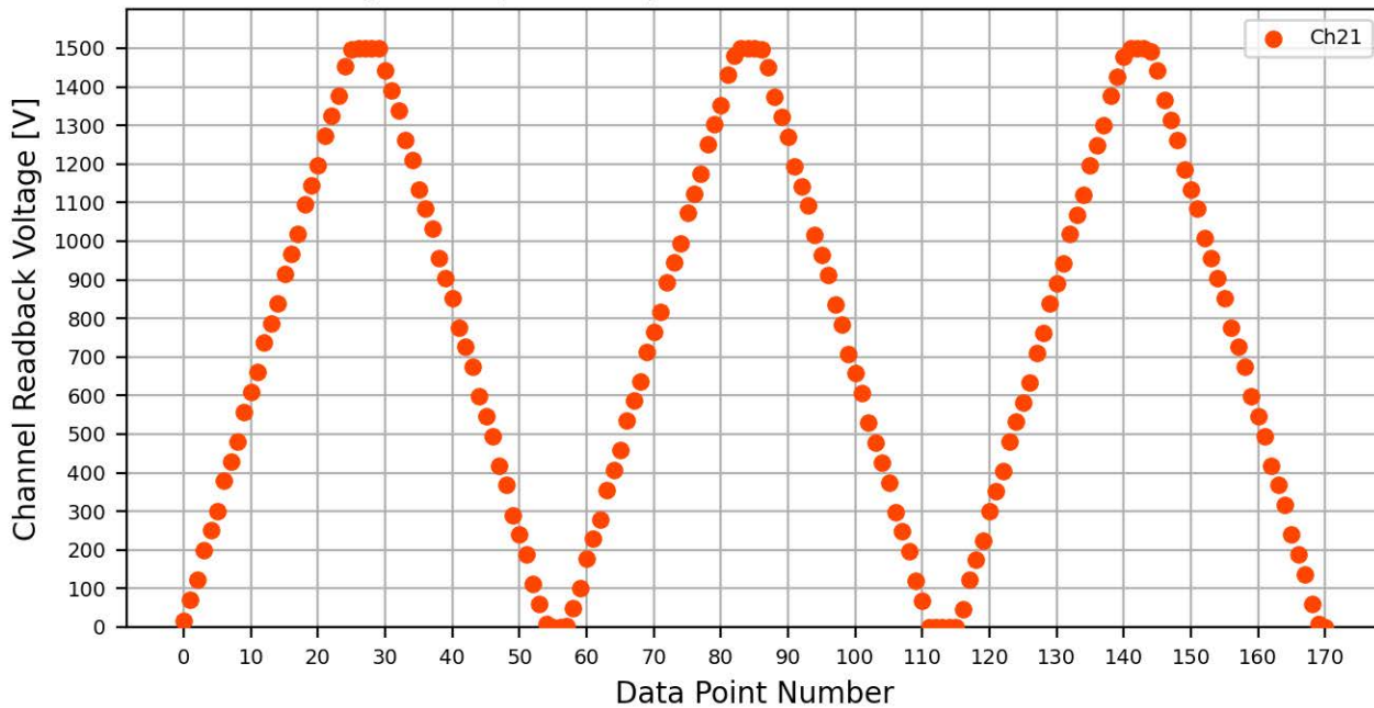
Voltage Ramp Test (Python) Bd #083, Slot #6, Ch #21
