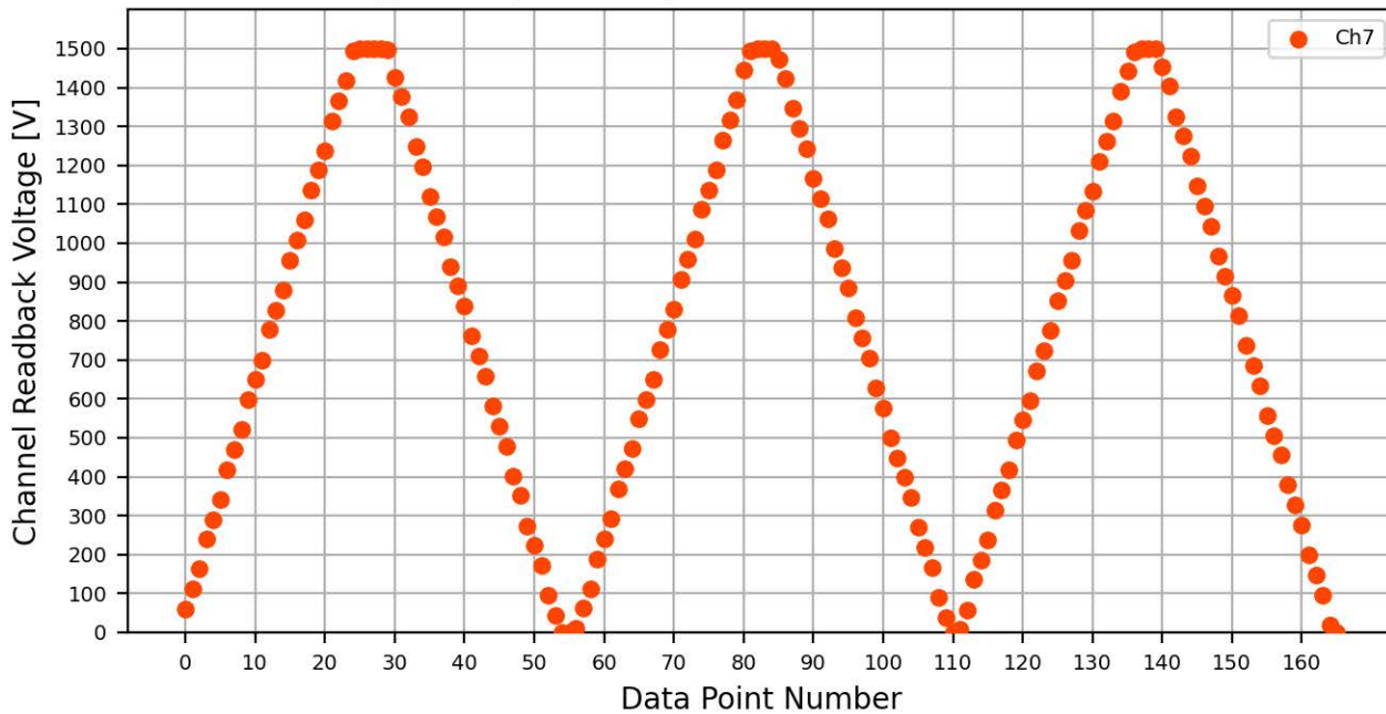
Voltage Ramp Test (Python) Bd #083, Slot #6, Ch #7
