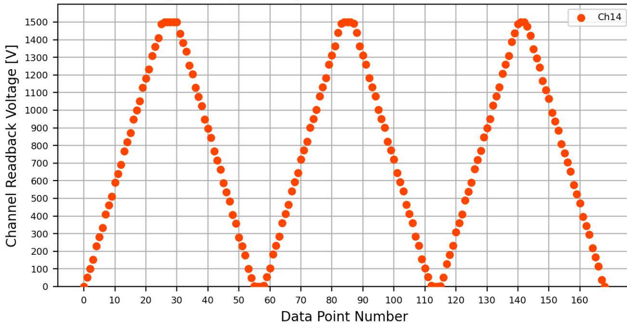
Voltage Ramp Test (Python) Bd #083, Slot #6, Ch #14
